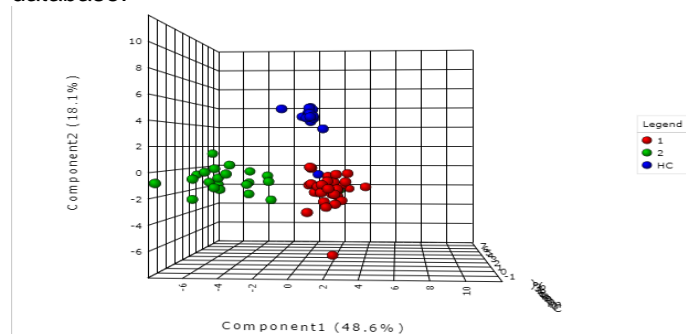
Image 2. Image of scores of the sPLS-DA models
