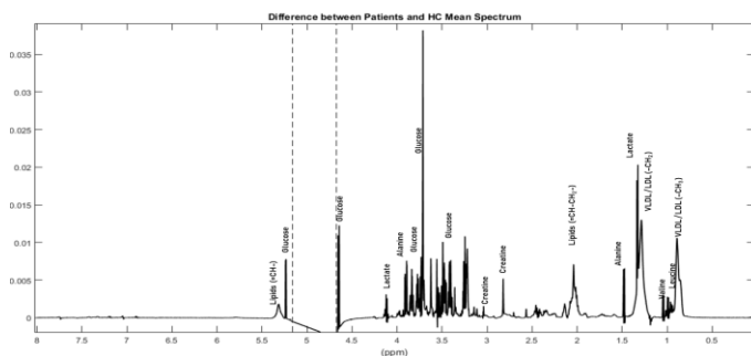
Image 1. Spectral differences among the mean control group ^1\text{H} -NMR subtracted from the mean crack users' ^1\text{H} -NMR spectra before treatment.
